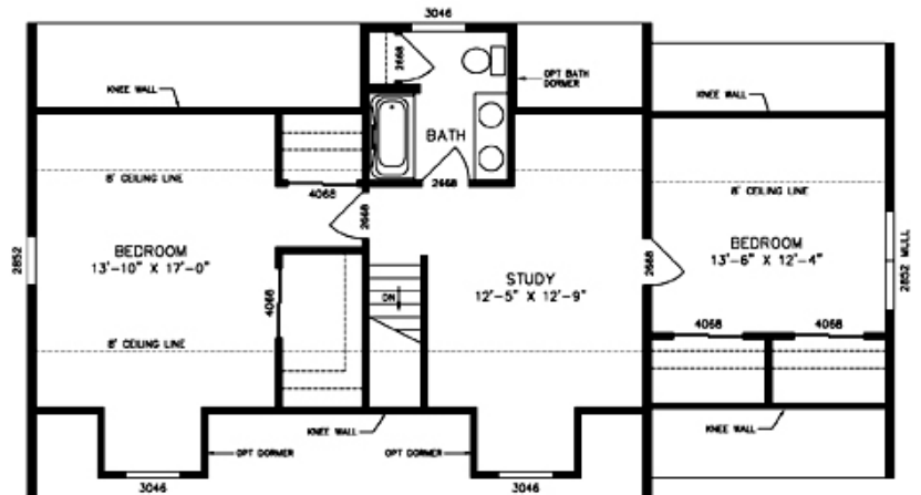
KILLINGTON PLAN No: NC6606 PROPOSED SECOND FLOOR (BY OTHERS) 17'0"/11'5" x 50'0"
