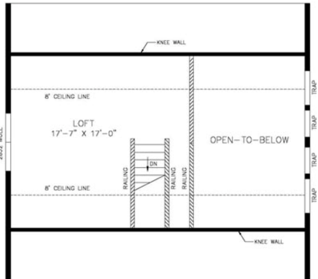
VALE PLAN NO: NC6601 PROPOSED SECOND FLOOR (BY OTHERS) 17'0" X 30'0"
