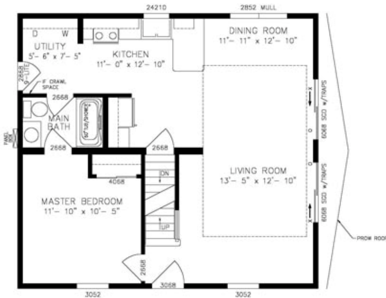
VALE PLAN NO: NC6601 FIRST FLOOR 27'4" X 30'0" 820 SQ. FT.
