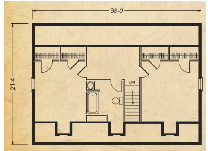
NORFOLK PROPOSED SECOND FLOOR 27'4" x 38'0"
