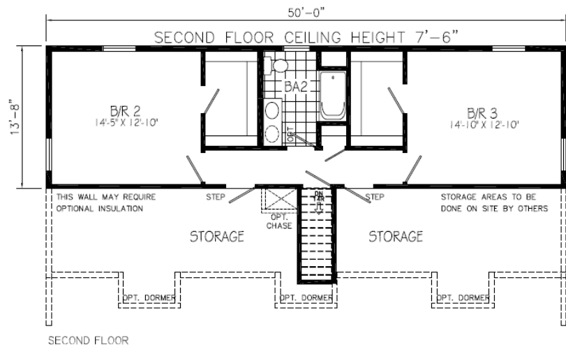
GEORGETOWN PLAN No: SB307A PROPOSED SECOND FLOOR (BY OTHERS)
