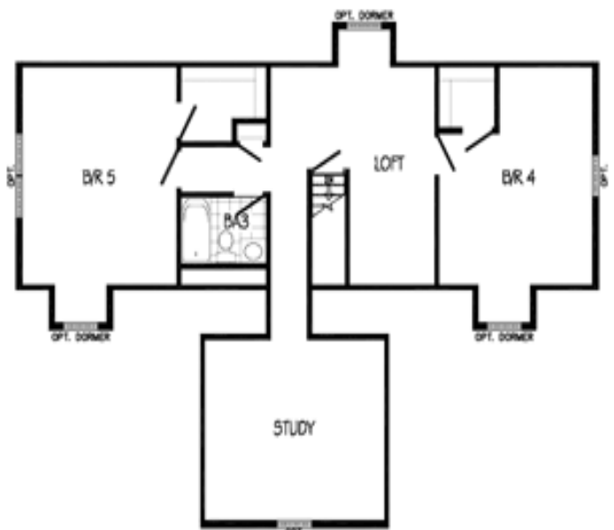
SHADOWBROOK PLAN No: ML501A PROPOSED SECOND FLOOR (BY OTHERS) APPROX. 1170 SQ. FT. UNFINISHED
