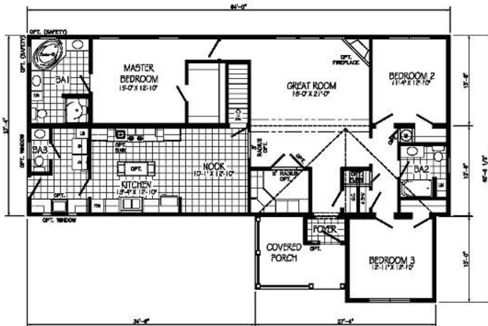
HELDERBURG PLAN NO: RL503A 41'0" x 64'0" 1959 SQ. FT.
