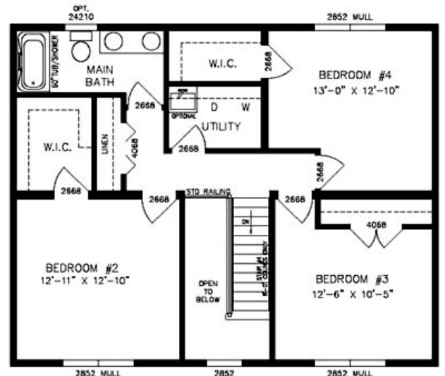
SPRING CREEK PLAN NO: NT6708 SECOND FLOOR 27'4" x 34'0"
