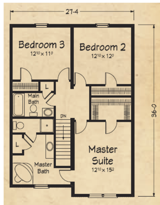
EDISTO SECOND FLOOR
