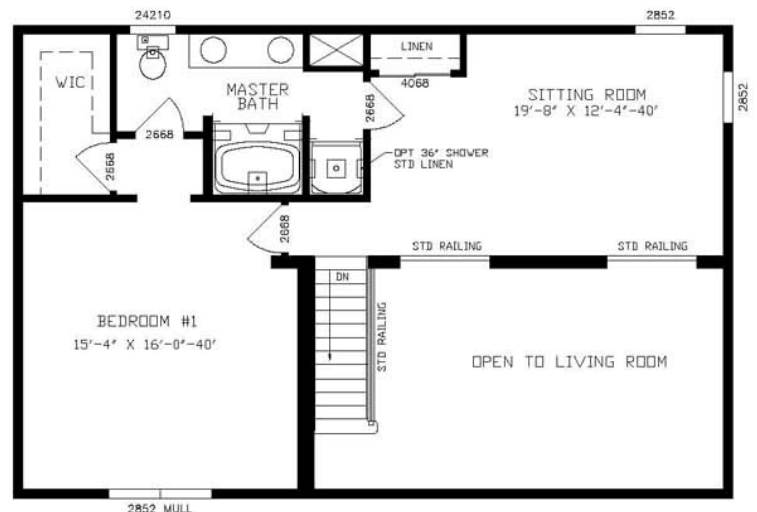
ASPEN II PLAN No: PT5024 SECOND FLOOR 26'4" x 44'0"
