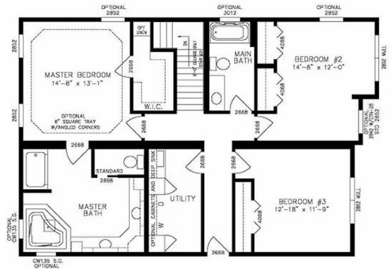
OPTIONAL SECOND FLOOR "B"
