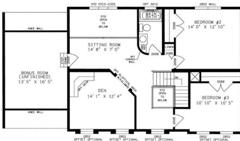
CHATHAM PLAN NO: PT5748 SECOND FLOOR 27'4" x 38'0"
