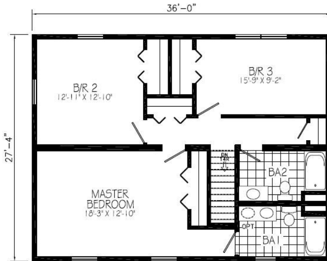
SECOND FLOOR
